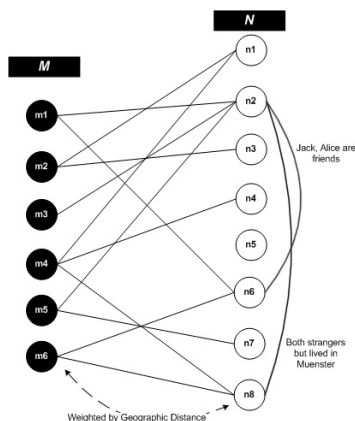
Fig. 1. An affiliation network of volunteers N and the VGI they contribute M with links between a volunteer and VGI entities weighted by distance between the volunteers and the observed entity's actual location. Links connecting N white nodes are a separate agent-agent social network, making this model a hybrid affiliation-one mode social network.
